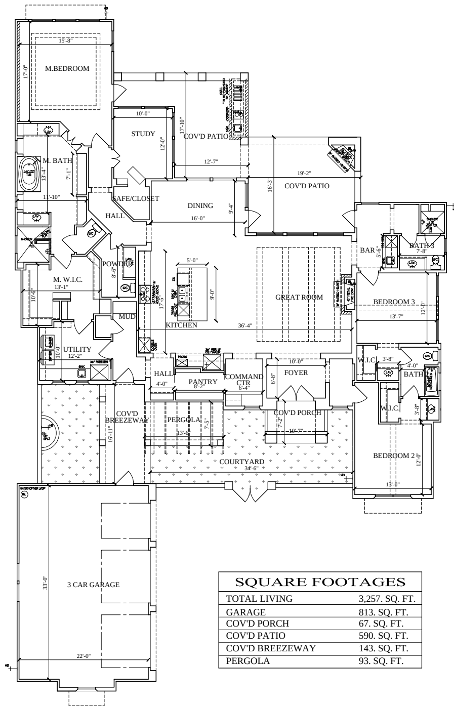
FLOOR PLAN
