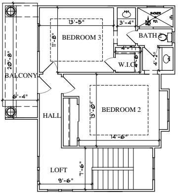
2ND FLOOR PLAN
