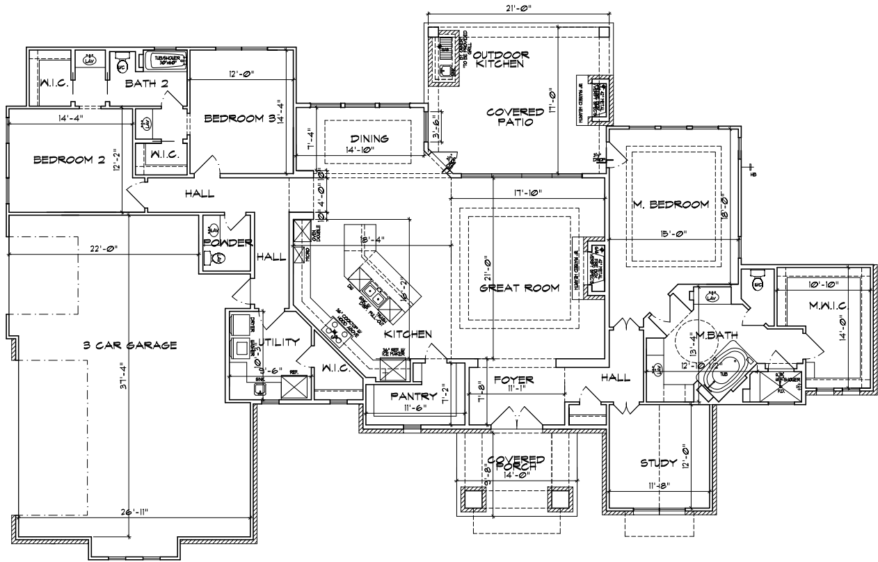
FLOOR PLAN
