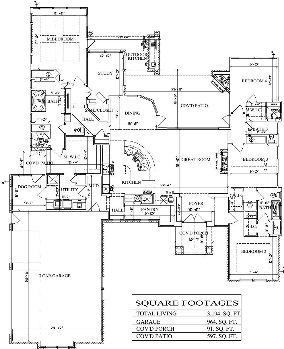
FLOOR PLAN
